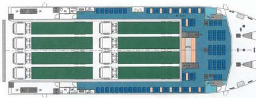
PASSENGER DECK
