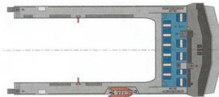
WHEELHOUSE DECK
